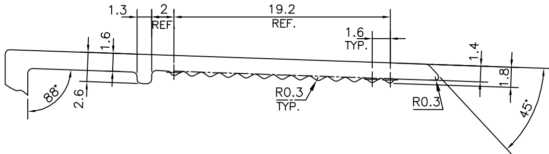
DETAIL OF "A" SCALE 3:1
