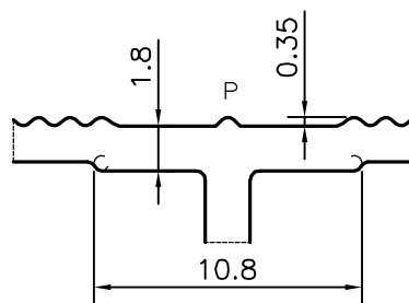
DETAIL OF "A" SCALE 3:1
