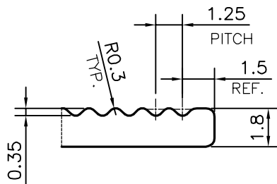
DETAIL OF "A" SCALE 4:1
