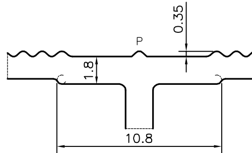
DETAIL OF "B" SCALE 4:1
