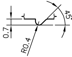
DETAILS OF "A" SCALE 4:1
