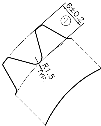
DETAIL OF "A" SCALE 2:1
