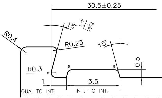
DETAIL OF "A" SCALE :- 8:1
