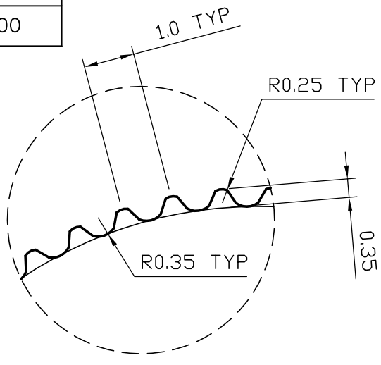
DETAIL-Z SCALE 10:1
