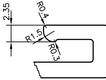
DETAIL "A" SCALE 3:1
