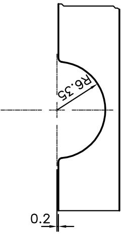
DETAIL OF "A" SCALE 2:1
