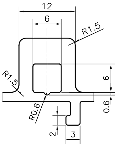
DETAIL OF "A" SCALE 2:1
