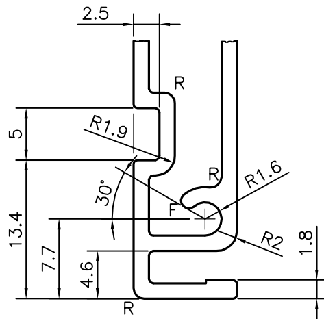
DETAILS OF "A" SCALE 2:1
