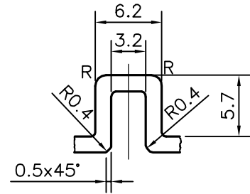
DETAILS OF "B" SCALE 2:1
