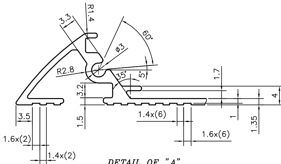
DETAIL OF "A" SCALE 2:1
