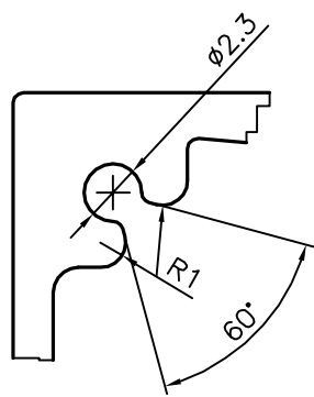
DETAIL "A" SCALE 3:1
