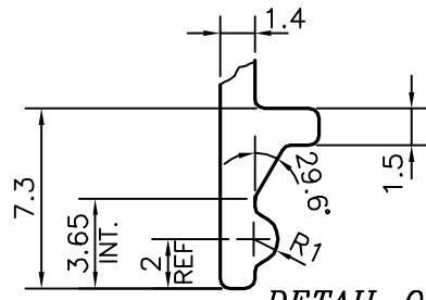
DETAIL OF "B" SCALE 2:1
