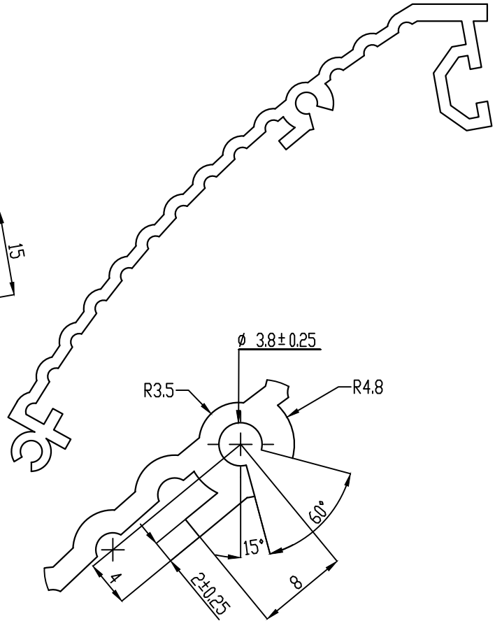
DETAIL B SCALE 3 : 1
