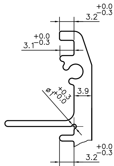
DETAIL OF "B" SCALE 2:1
