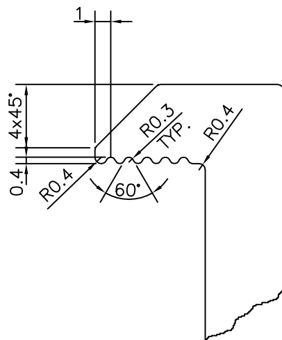
DETAIL OF 'A' SCALE 3:1
