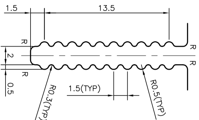
DETAIL OF "A" SCALE 4:1
