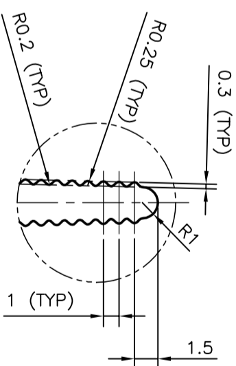
DETAIL OF "B" SCALE 3:1
