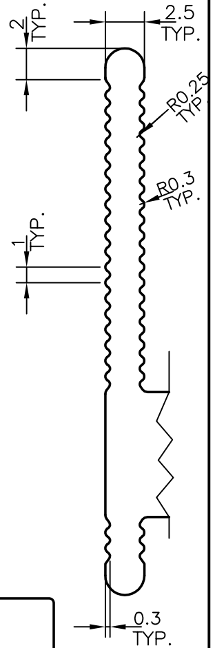
DETAIL OF "A" SCALE 3:1
