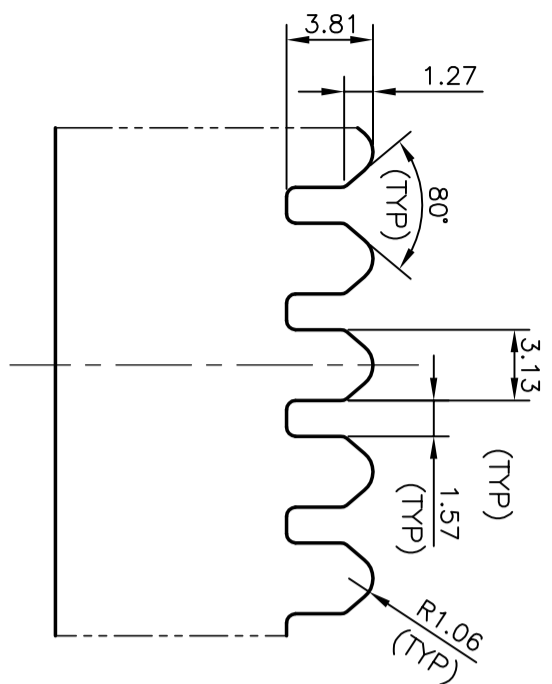
DETAIL OF "A" SCALE 3:1
