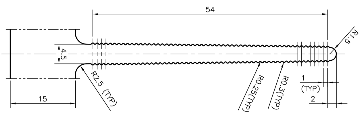
DETAIL OF "B" SCALE 2:1
