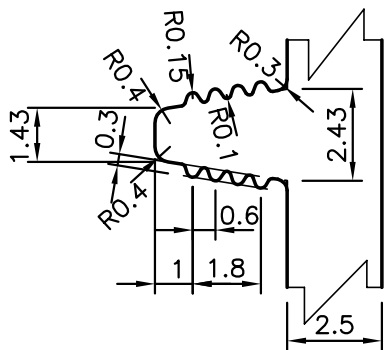
DETAIL OF "A" SCALE 5:1
