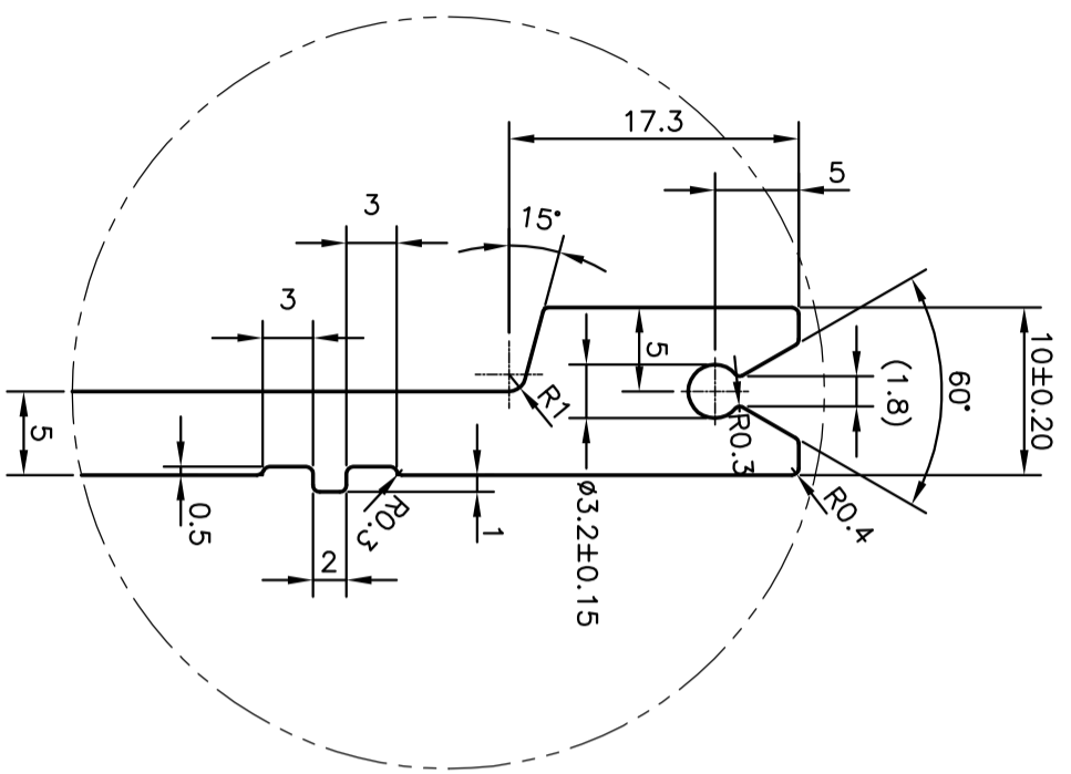
DETAIL OF "B" SCALE 2:1
