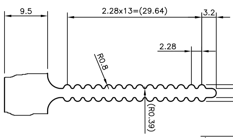
DETAIL OF "A" SCALE 2:1
