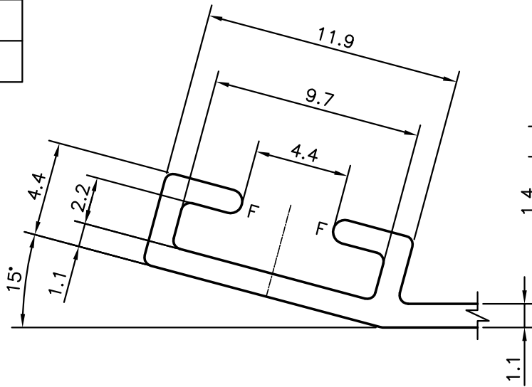
DETAIL OF "A" SCALE 4:1
