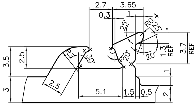
DETAIL OF "A" SCALE 4:1
