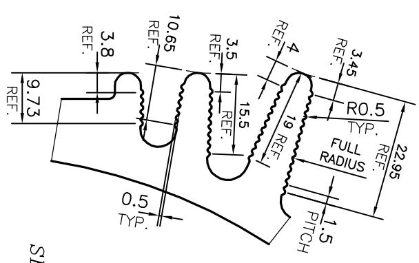
SERRATION DETAIL SCALE 1:1
