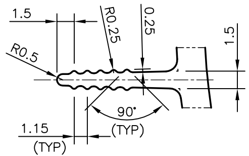
DETAIL OF "A" SCALE 3:1
