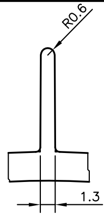
DETAIL OF "A" SCALE 3:1
