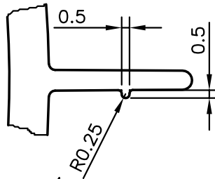
DETAIL OF "B" SCALE 3:1
