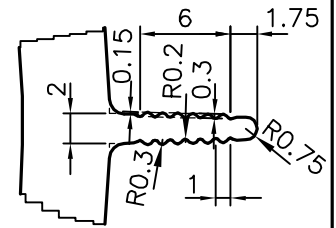
DETAILS OF "A" SCALE 2:1
