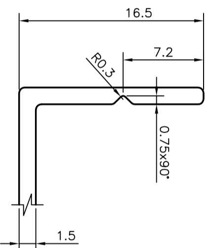
DETAIL OF "A" SCALE 3:1
