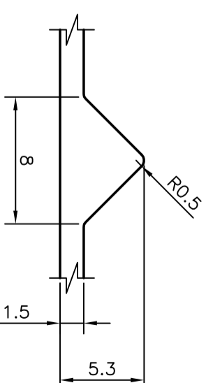
DETAIL OF "B" SCALE 3:1
