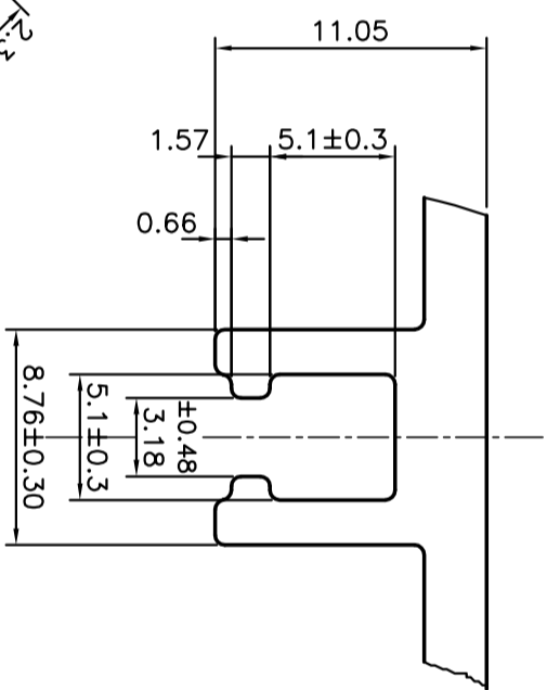
DETAIL "C" (3:1)
