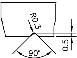
DETAILS OF 'V' GROOVE SCALE 1:3
