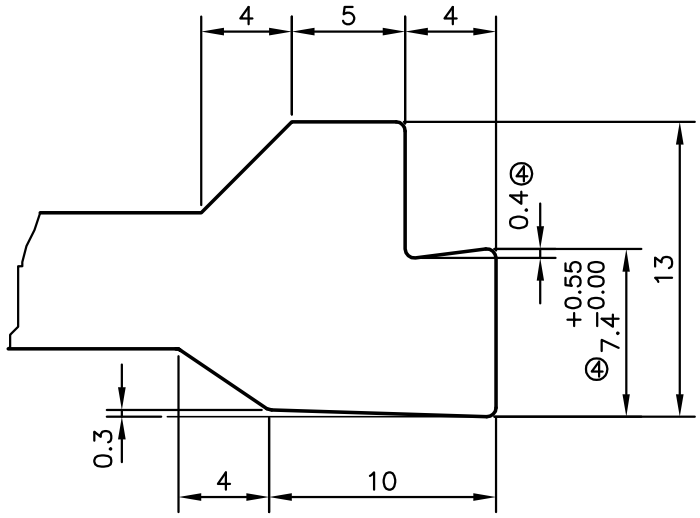
DETAIL "A" SCALE 3:1
