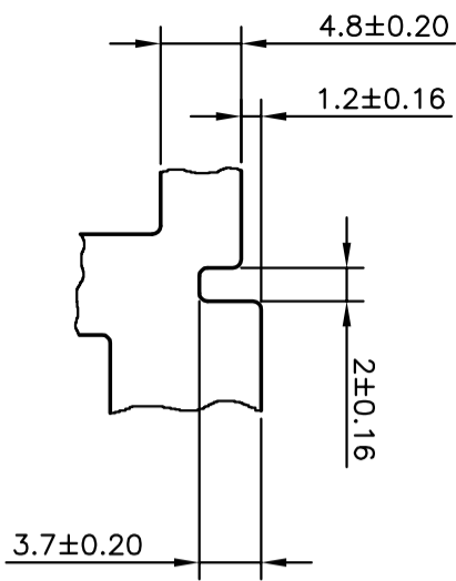
DETAILS OF "B" SCALE 2:1
