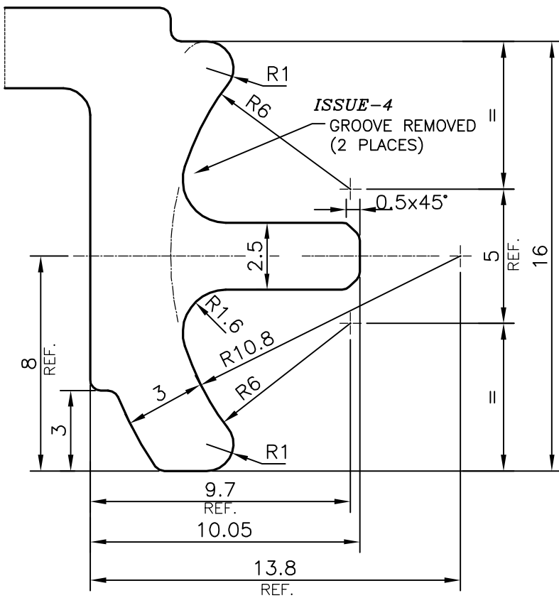
DETAIL OF "A" SCALE 5:1
