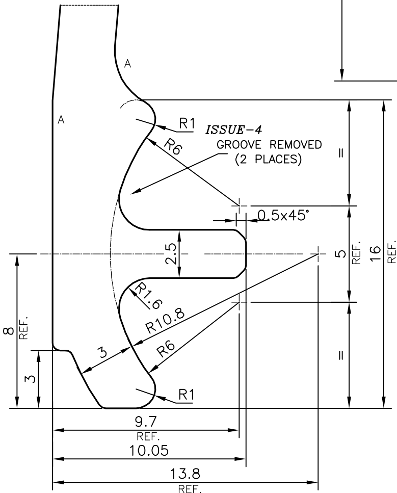
DETAIL OF "A" SCALE 5:1
