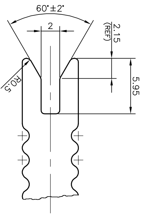
DETAILS OF "A" SCALE 4:1
