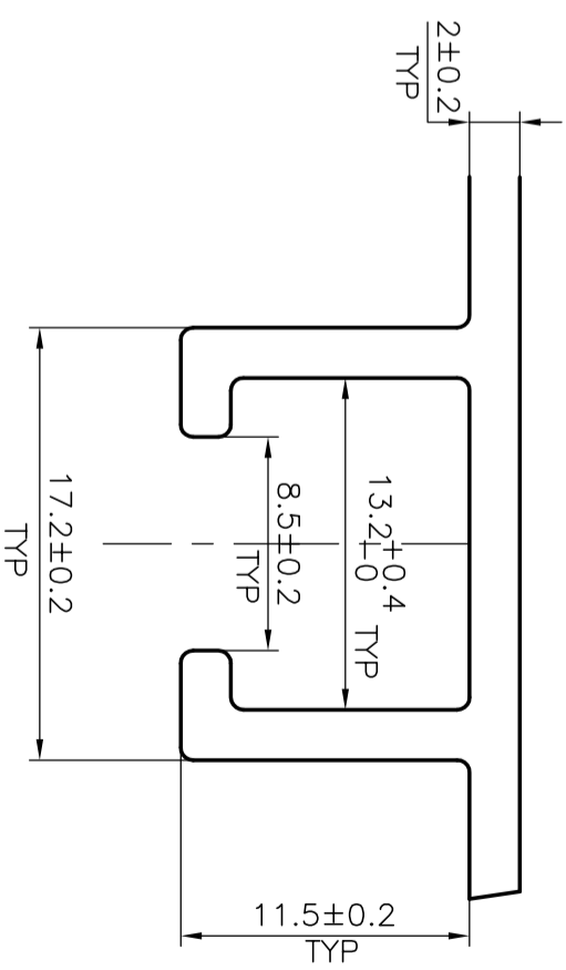
DETAIL "A" SCALE 3:1
