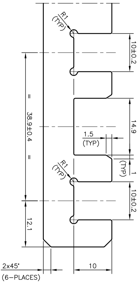
DETAIL OF "B" SCALE 2:1
