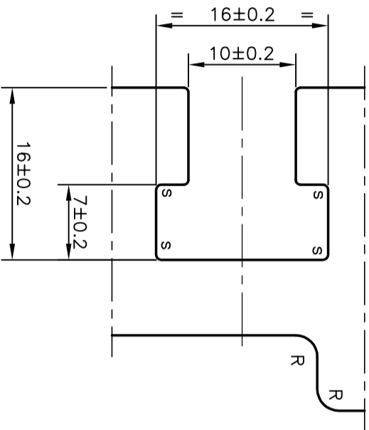
DETAIL OF "A" SCALE 2:1 (4 PLACES)
