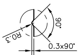
DETAIL OF "C" SCALE 3:1
