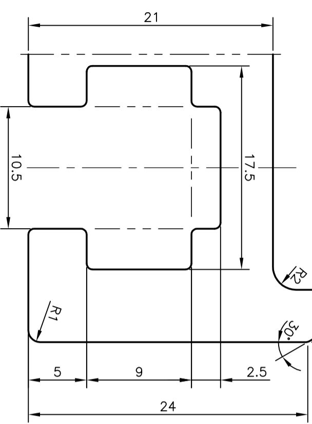
DETAIL OF "A" SCALE 3:1
