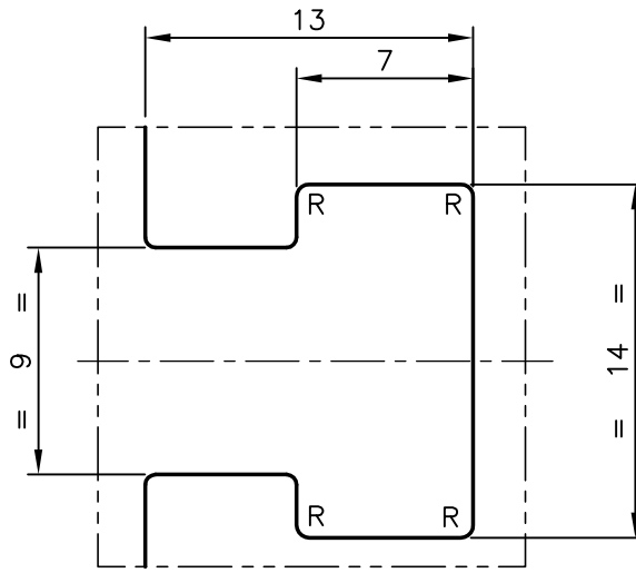
DETAIL OF "A" SCALE 3:1 (3 PLACES (TYP) )
