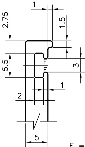
DETAIL OF "A" SCALE 2:1
