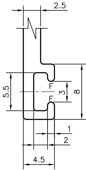
DETAIL OF "A" SCALE 3:1
