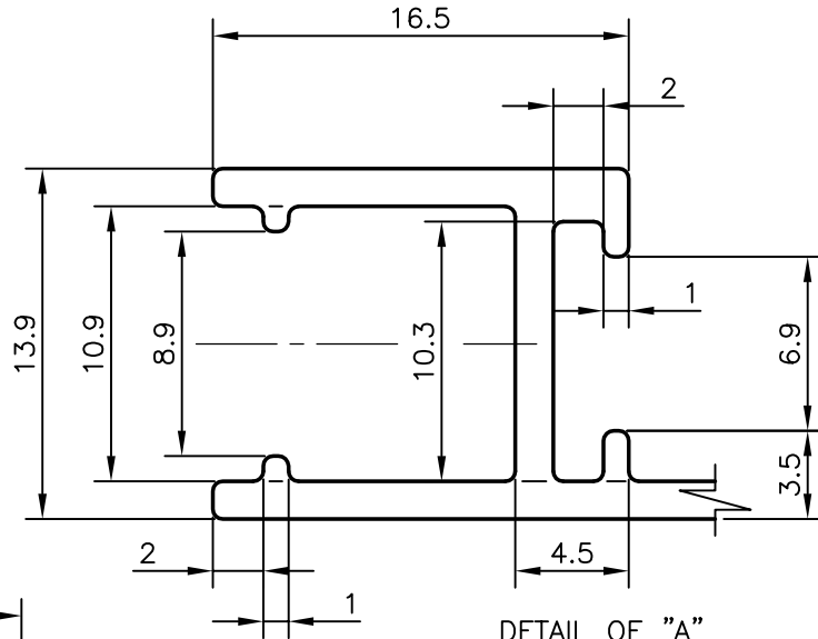
DETAIL OF "A" SCALE 3:1
