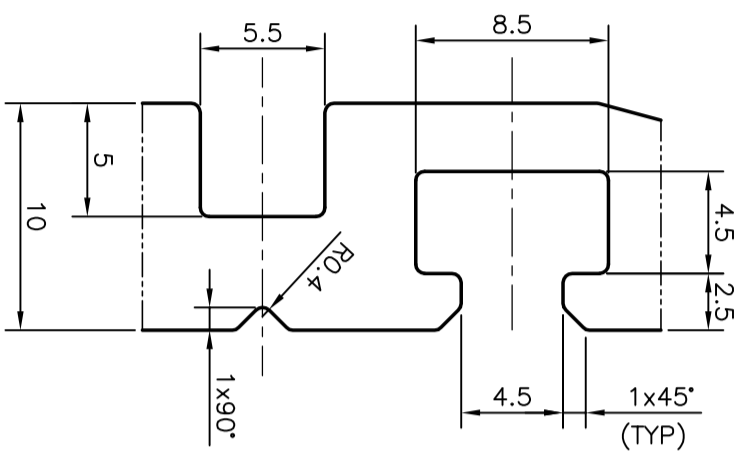
DETAIL OF "A" SCALE 3:1
