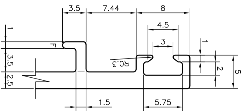
DETAIL OF "A" SCALE 3:1
