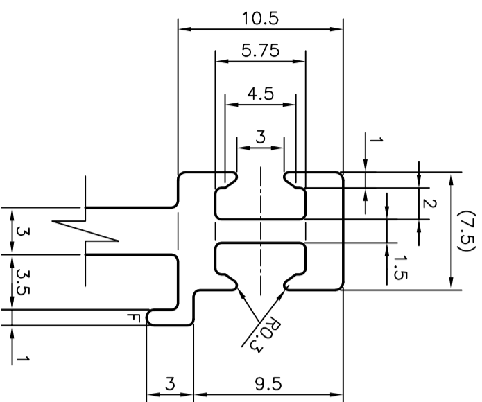
DETAIL OF "B" SCALE 3:1
