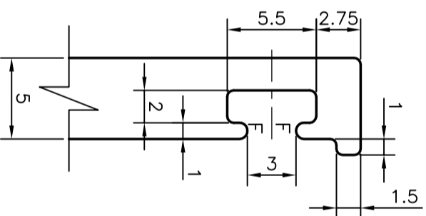
DETAIL OF "A" SCALE 3:1
