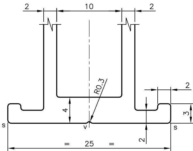
DETAIL OF "A" SCALE 3:1
