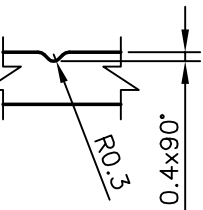
DETAIL OF "C" SCALE 3:1
